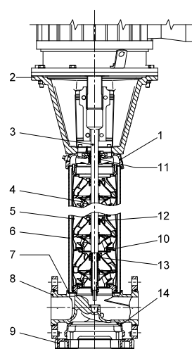
Sectional drawing
