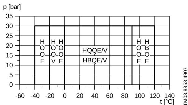
Fig. 7 Operating range of standard shaft seals
