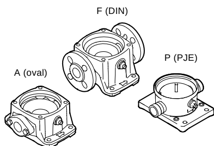
Fig. 13 Pump connections
