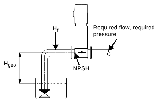
Fig. 11 Dimensional data
